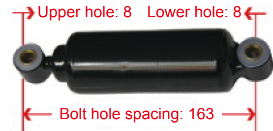
Black Universal Seat Shock Absorber
