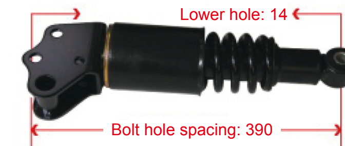
D215221440540 New M3000 Rear Shock Absorber Bracket
