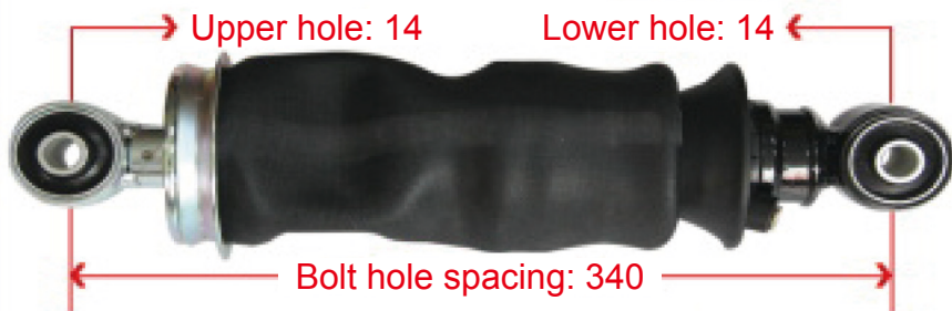
5001315-E18 Tianwei Rear Air Bags
