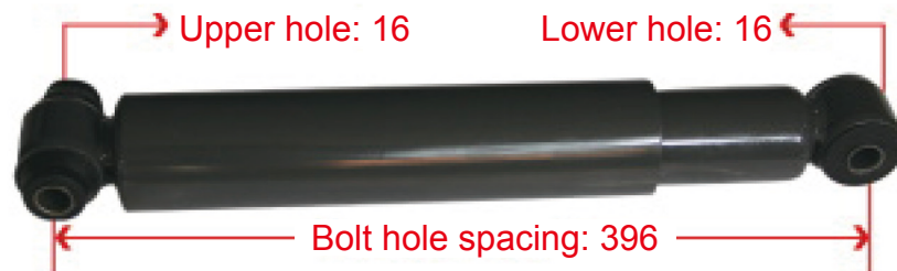
WG9925680031 TX Front Axle Shock Absorber
