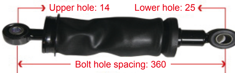
YG1671430032 MAX Front Heavy-Duty Air bags
