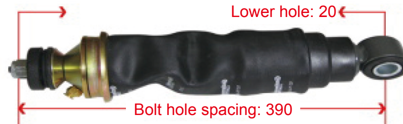
WG1664430078 A7 Front air bags
