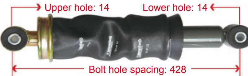
WG1664440068 A7 Rear air bags
