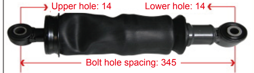
712W41722-6031 TX Rear Air Bags
