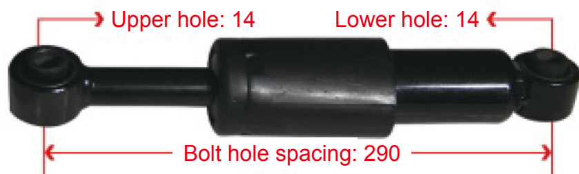
YG1671440042 MAX Transverse Shock Absorber
