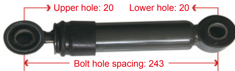
WG1642440021 HOWO Transverse Shock Absorber
