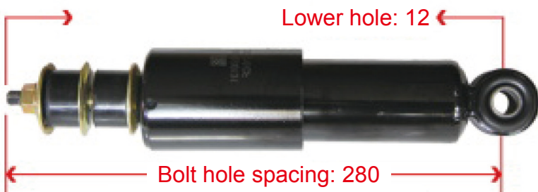
1B24950200131 Auman ETX Front Shock Absorber
