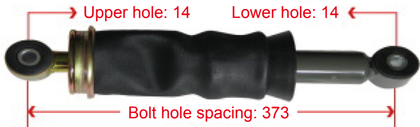
WG1671430192 Haohan N7G Front Air Bags
