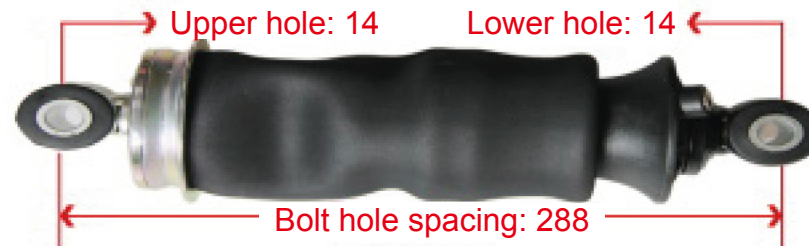
D214251440020 X3000 Rear Air Bags
