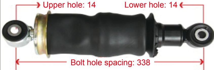
500131SA1063-C00 JH6 Rear Air Bags
