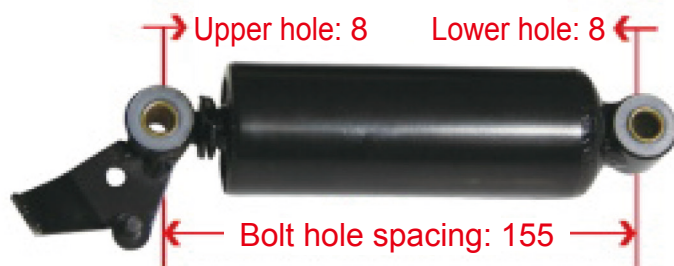
WG1662510145 A7Seat Shock Absorber
