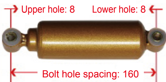
Yellow Seat (Long Type) Seat Shock Absorber
