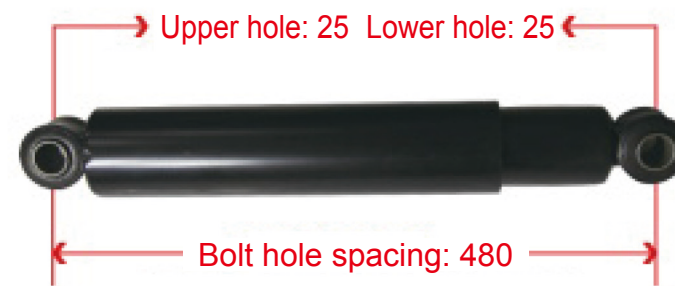
D295259680103 M3000 Rear Axle Shock Absorber
