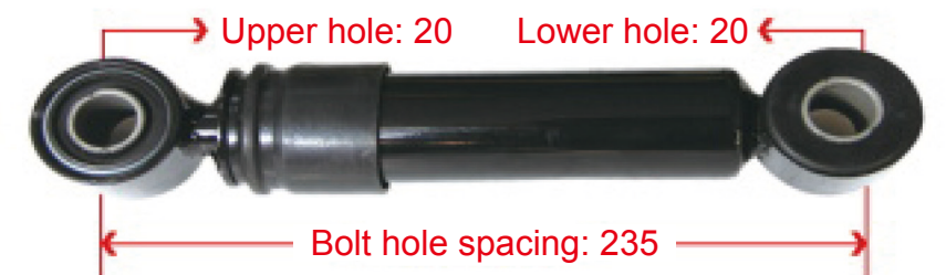
D213241440080 X3000 Transverse Shock Absorber
