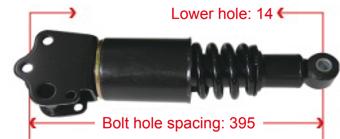
D215221440580 M3000 Rear Shock Absorber
