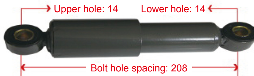
WG1642430091 HOWO 08 Longitudinal Shock Absorber
