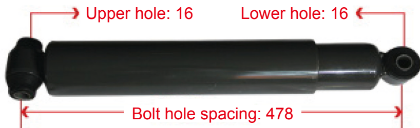
WG9725680014 T5G Front Axle Shock Absorber
