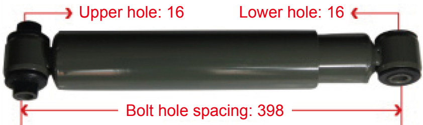
WG9531680032 Haohan Front Axle Shock Absorber
