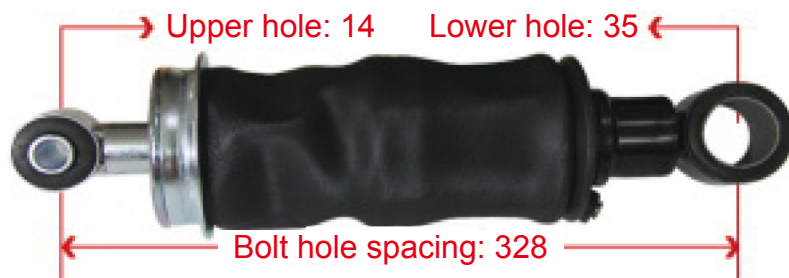
H4502A01030A0 GTL Front Large Bore Air Bags
