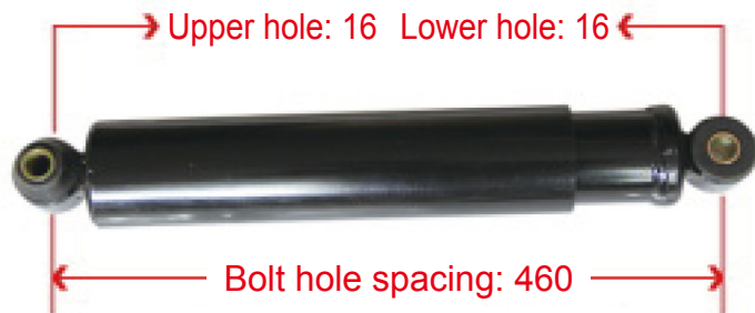
1124029200005 Auman ETX Front Axle Shock Absorber
