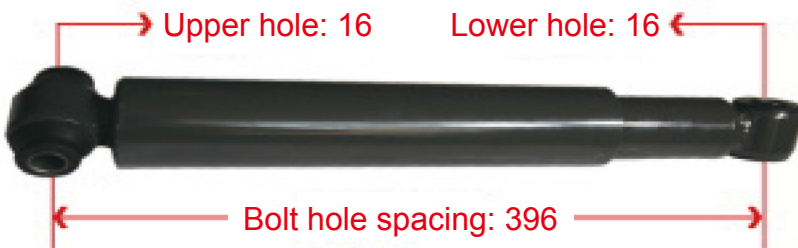
WG9925680031 T7 Front Axle Shock Absorber
