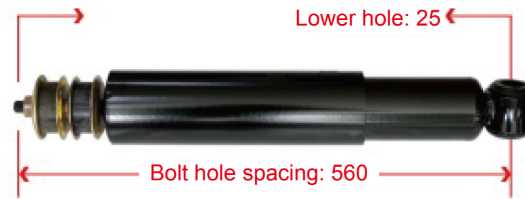
XG2921WLFWL11-010 XCMG Front Axle Shock Absorber
