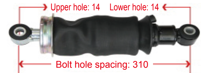
NXG50NMBW111-01042 XCMG G5 Rear Air Spring
