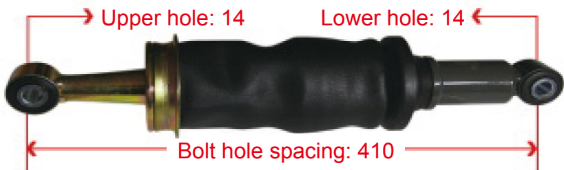
WG1671430119 Haohan Front Air Bags
