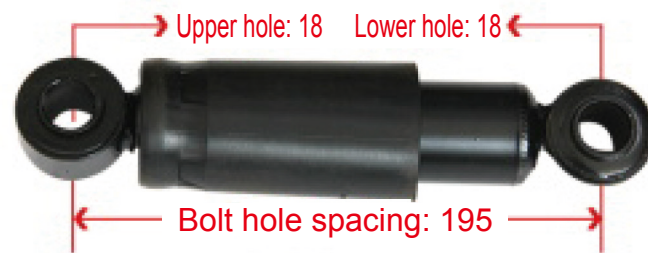
0606912205-6048 Mercedes-Benz Cab Shock Absorber (Small)
