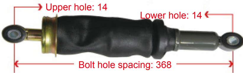
WG1671440180 Haohan Rear Air Bags
