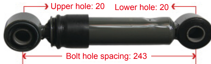
WG164440021 Haohan Transverse Shock Absorber
