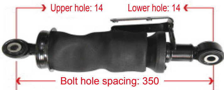
5001315-10638-C00 JH6 Rear Air Bags with Bracket (1301B)
