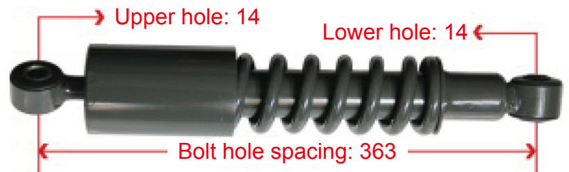
WG1654440010 Haohan Rear Shock Absorber
