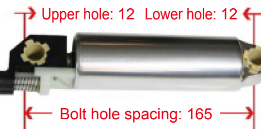
Adient Seat Shock Absorber (Black Bracket)
