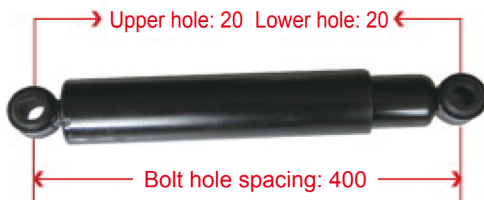
1122929200005 Auman ETX 1st Front Axle Shock Absorber
