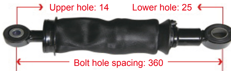
YG1671430034 MAX Front air bags
