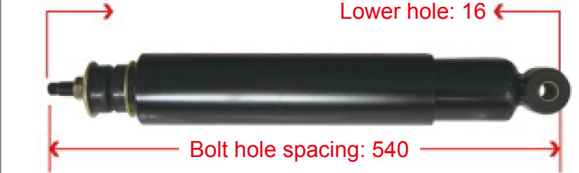
D295259680012/9680013 F3000 Front Axle Shock Absorber
