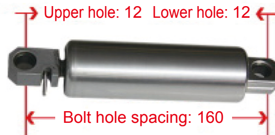
Grammer Slim Seat Shock Absorber
