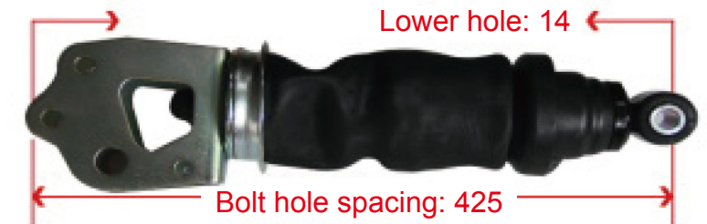
D214251440060 X3000 Rear Air Bags with Bracket
