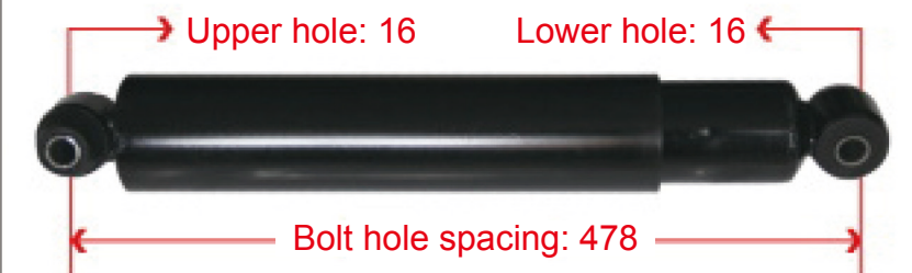
D219912680014 F3000 Front Axle Shock Absorber
