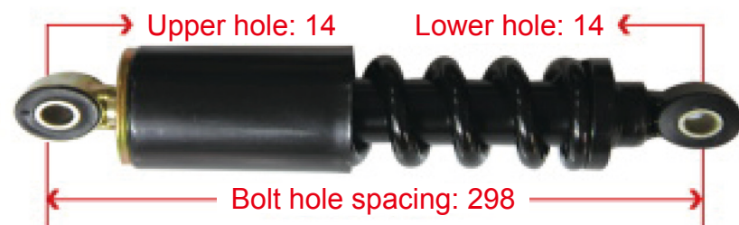
D213241440150 Delong Rear Shock Absorber
