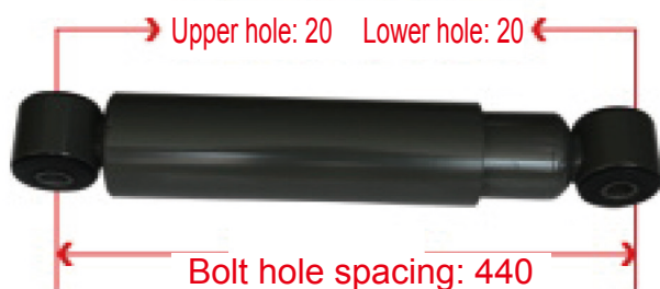
2915010A001A0 Liuqi Rear Axle Shock Absorber
