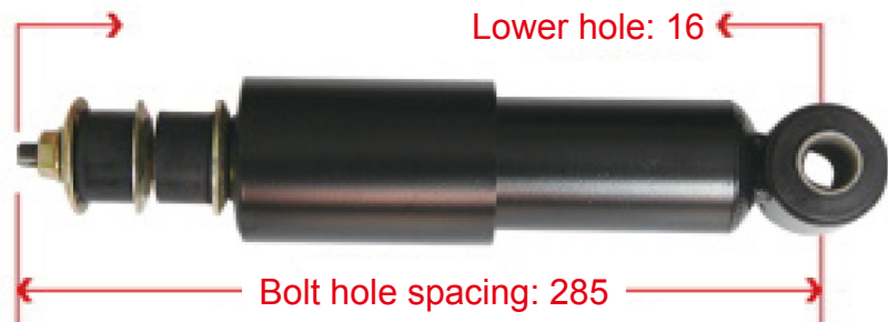
5001020-D850 Xindawei Front Shock Absorber
