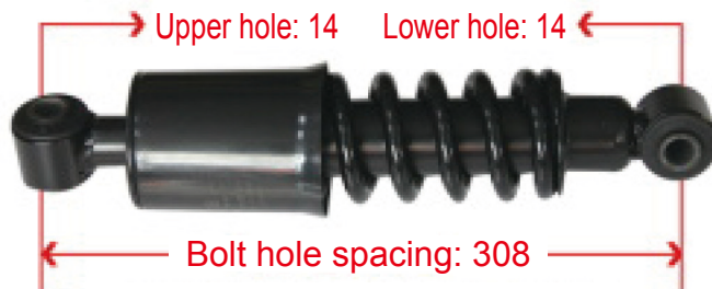
5001320-18T-C00 New JH6 Rear Shock Absorber
