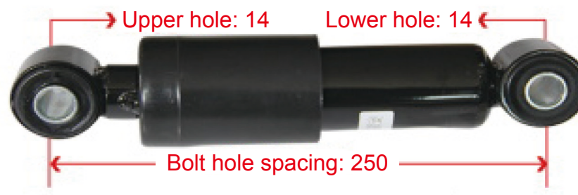
H4502B01016A0 GTL Transverse Shock Absorber
