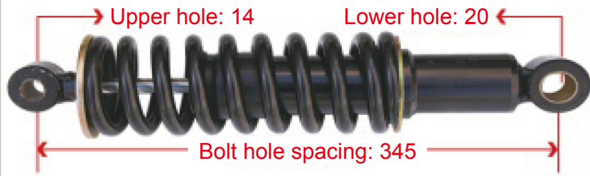
5001085-C1102 Dongfeng Tianjin Front Cab Shock Absorber
