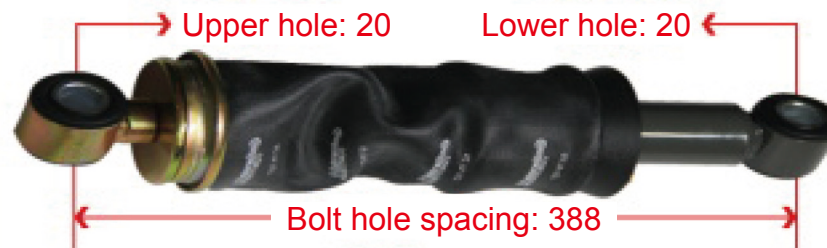
WG1664430120 T7 Front Air Bags
