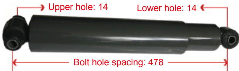
WG9725680014 Haohan Front Axle Shock Absorber
