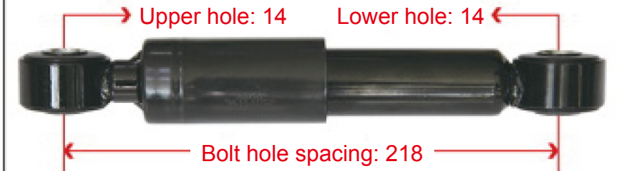
50WLAM111-01054 XCMG Transverse Shock Absorber
