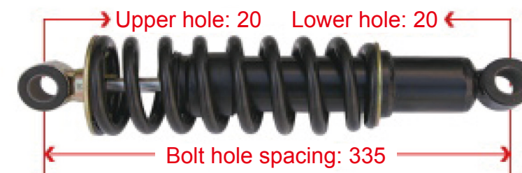
5001085-C1800 New Dongfeng Tianjin Front Cab Shock Absorber
