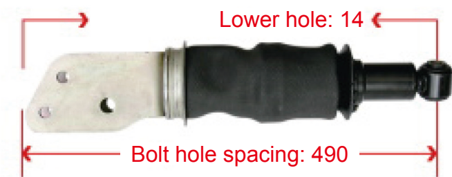
NXG50WBLW231-01153 XCMG Rear Air Spring
