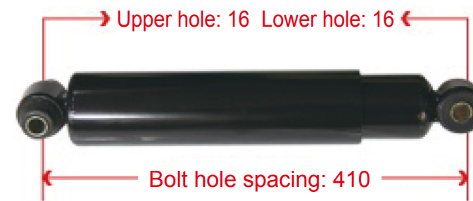
D296319680103 M3000 Front Axle Shock Absorber
