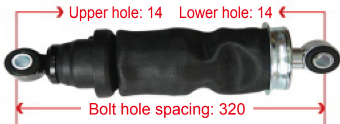
5001220-D850 Xindawei Rear Air Bags
