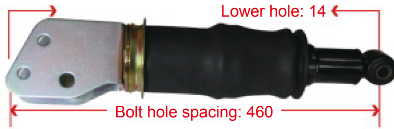
H4503050201A0 EST Rear Air Bags
