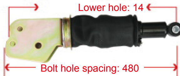
NXG50WBLW111-01153 XCMG G7 Rear Air Spring
