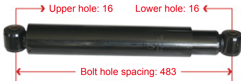
004423 9800 Mercedes-Benz Front Axle Shock Absorber
