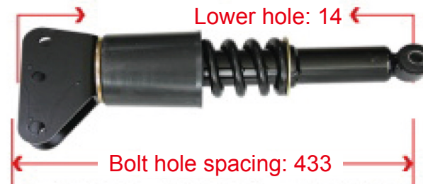
50WLFW541-01053 XCMG Rear Cab Shock Absorber
