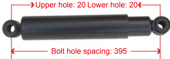
2921 C-010-A Dongfeng 145 Front Axle Shock Absorber
