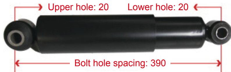
DZ9X259680003 X3000 Delong Front Axle Shock Absorber
