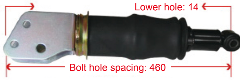
H4502B01015A0 GTL Rear Air Bags
