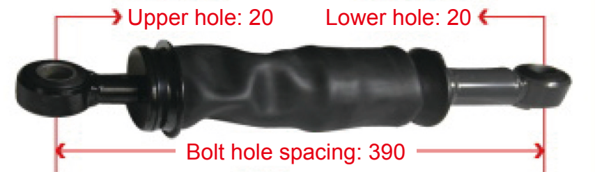
WG1664430201 T7 Front Air Bags
