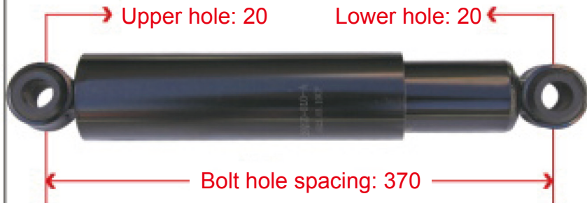
29210-010-A Dongfeng 140 Front Axle Shock Absorber
