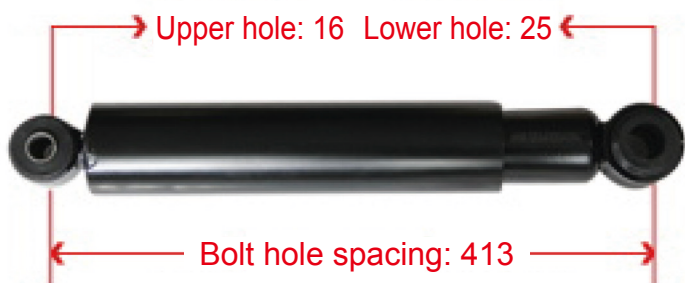
H4292070105A0 Auman ETX New Model Front Axle Shock Absorber
