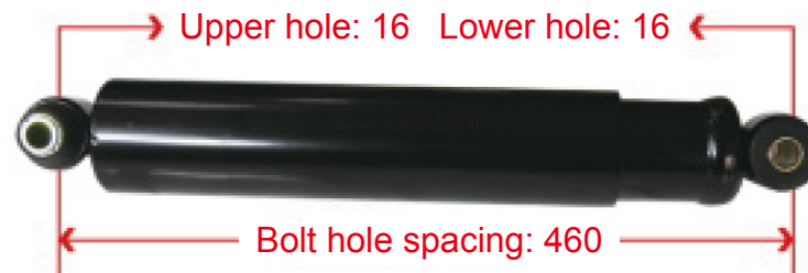
D295259680640 X3000 Front Axle Shock Absorber
