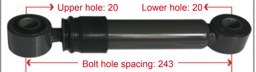
WG1664440100 T5G Transverse Shock Absorber
