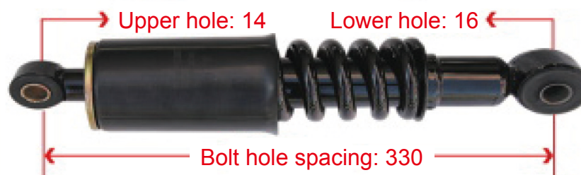
5001082-C5800 Dongfeng KR Front Cab Shock Absorber
