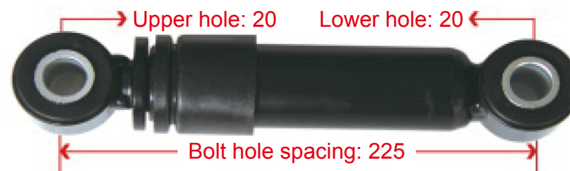
D214251440480 Delong Transverse Shock Absorber
