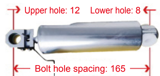
CVG Seat Shock Absorber
