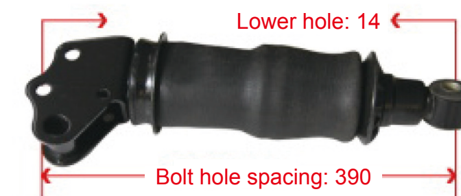
D215221440880 New M3000 Rear Air Bags Bracket
