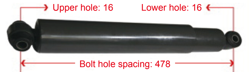
WG9925680028 T7 Front Axle Shock Absorber
