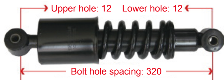
M4Q-5001250B Liuqi Balong Rear Cab Shock Absorber
