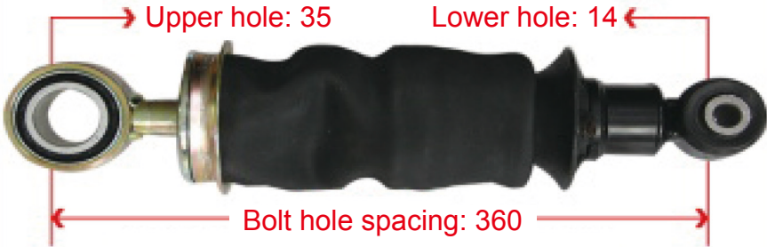
5001025A1063-C00 JH6 Front Air Bags
