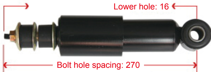
5001020-D488 Xindawei Front Shock Absorber
