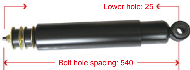
1120029200005 Auman ETX 2nd Front Axle Shock Absorber
