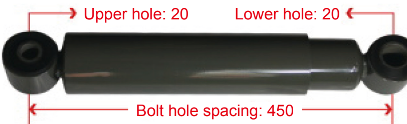
WG9925688101 T7 Front Axle Shock Absorber
