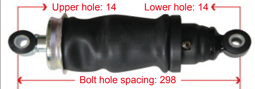
81.41722.6052 F3000 Rear air bags
