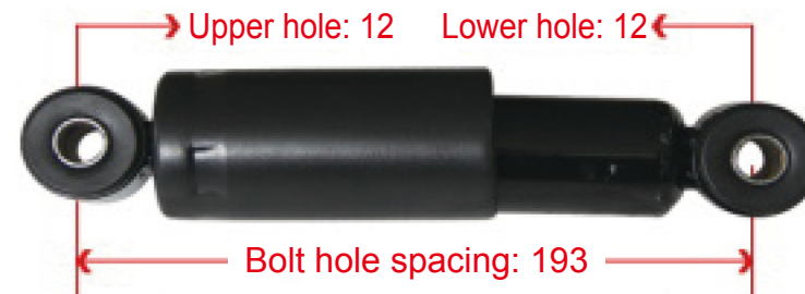
H4502A01316A0 GTL Front Cab Shock Absorber
