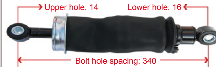
5001086-C3300 Dongfeng Tianlong Modified Front Air Bags
