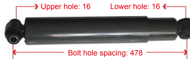
WG9925680028 HOWO Front Axle Shock Absorber
