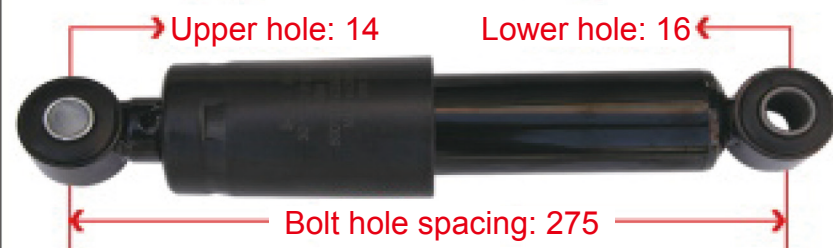
5001086-C3300 Dongfeng KL Front Cab Shock Absorber
