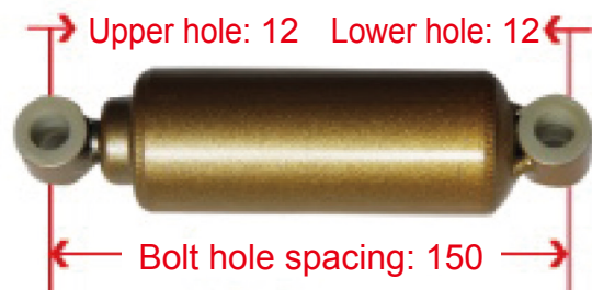
Yellow Seat (Large Hole) Seat Shock Absorber
