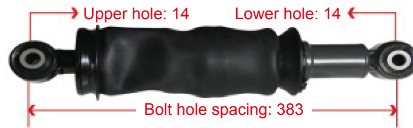
712W41722-6021 TX Front Air Bags
