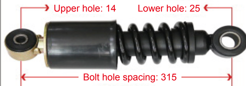
NXG50NMBW111-01070 XCMG Front Cab Shock Absorber
