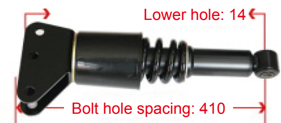
5188910405 Mercedes-Benz Rear Cab Shock Absorber
