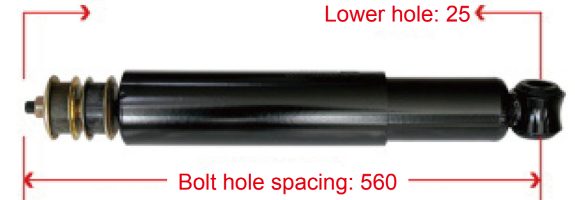
XGA2921LWFW251L XCMG Front Axle Shock Absorber
