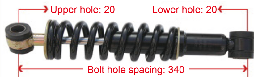
5001085-C1800 New Dongfeng tianlong Front Cab Shock Absorber
