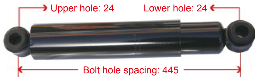
2921010-T0502 Dongfeng S50 Front Axle Shock Absorber
