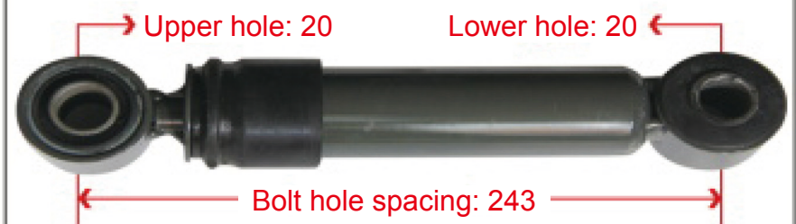
WG1642440021 HOWO 08 Transverse Shock Absorber
